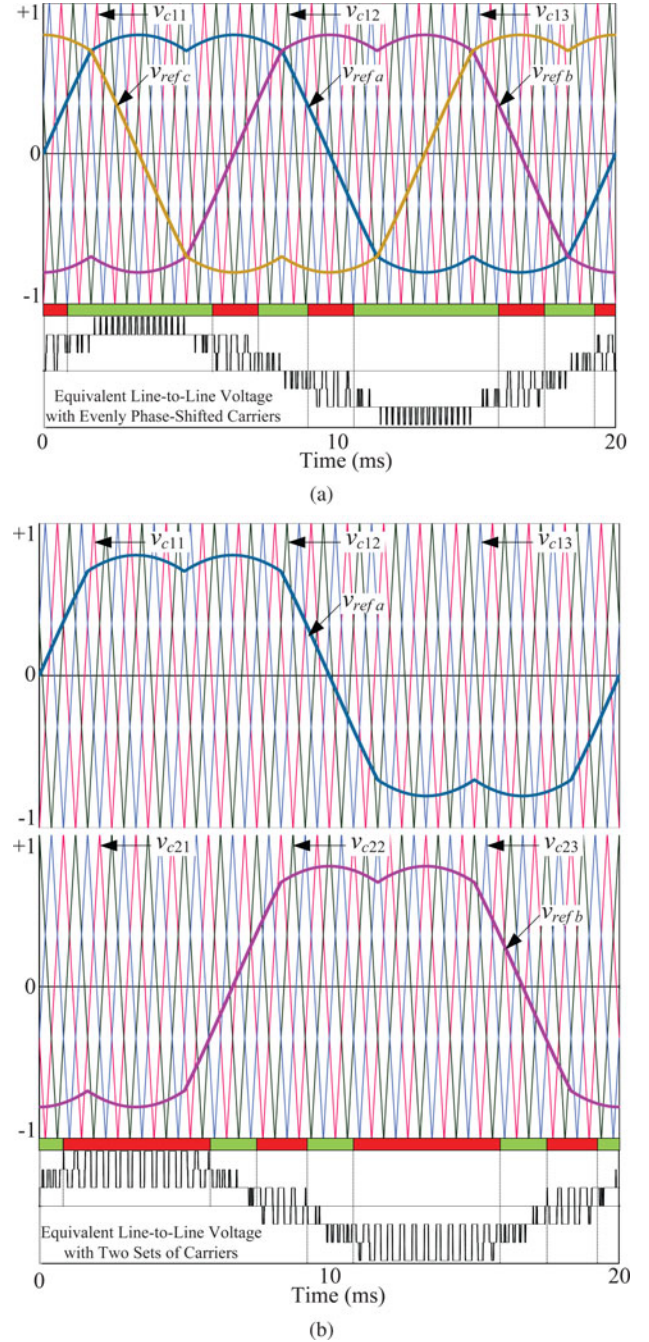
Fig. 2. Voltage references, set of carriers, and Thevenin-equivalent line-to-line output voltage ( v_{ab} ) for a three-phase VSI with three legs connected in parallel for m_a = 0.8 and f_c = 800 Hz: (a) one set of carriers and (b) two sets of carriers.
