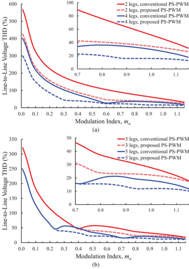
Fig. 6. Line-to-line THD versus modulation index for (a) two and four legs in parallel and (b) three and five legs in parallel.
