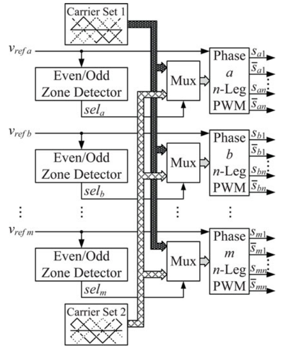
Fig. 5. Generalized m -phase n -leg modulator diagram.
