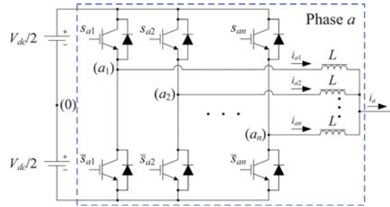
Fig. 1. One phase of a VSI incorporating n legs connected in parallel.
